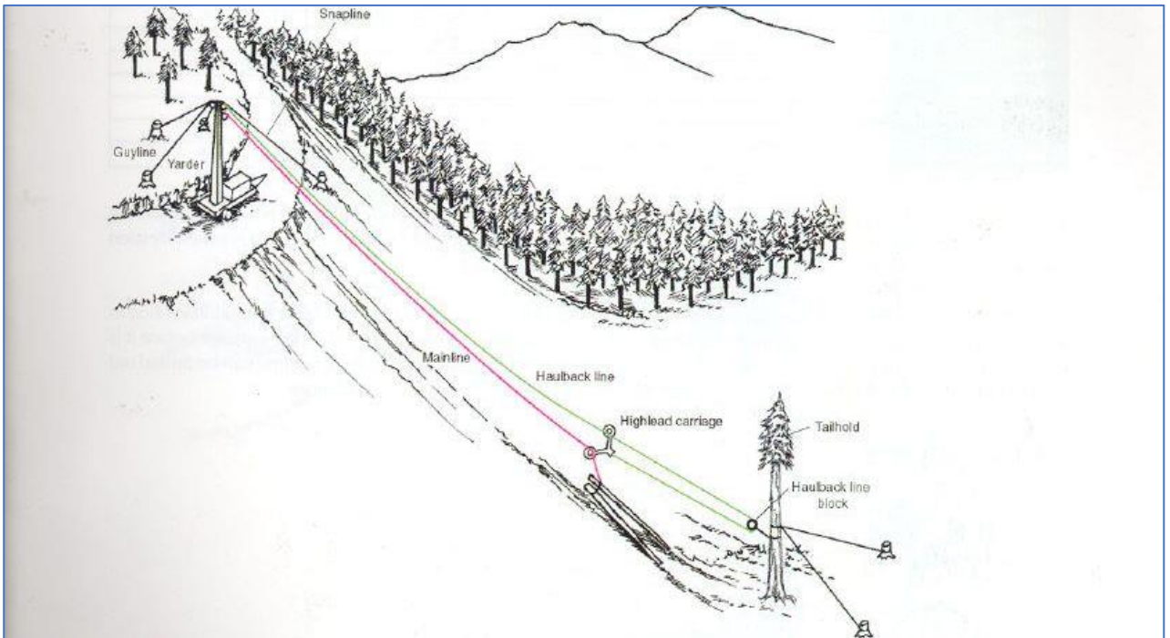
Figure 4: High-lead system with a carriage as used in South Africa. 8
