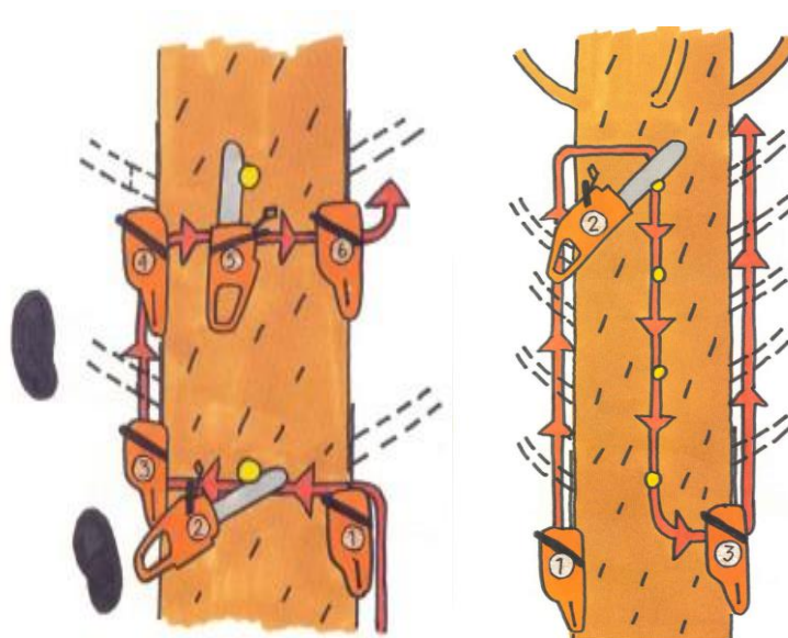
Figure 3: (left) six-point lever method and (right) sweep method 5
