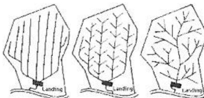
Figure 2: Skid trail layouts, left to right: parallel, herringbone, and dendritic design.
