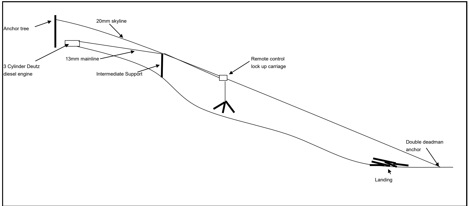
Figure 6: Concept design of a long-distance gravity skyline configuration.
