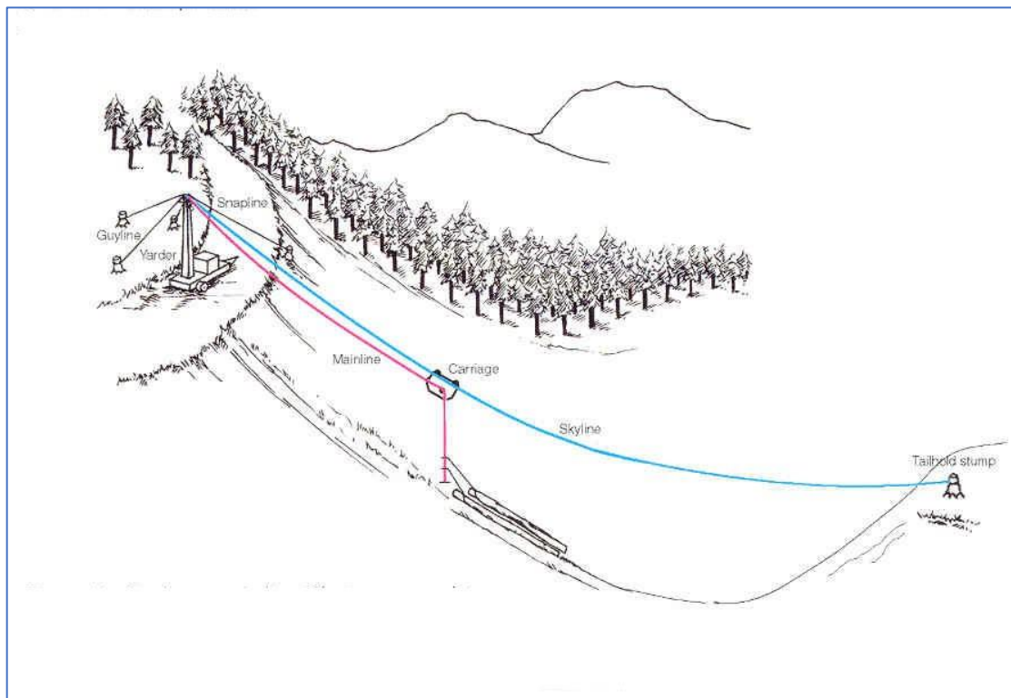
Figure 5: Standing skyline system. 8
