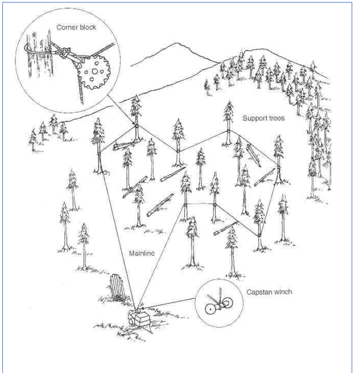
Figure 7: Monocable system. 8
